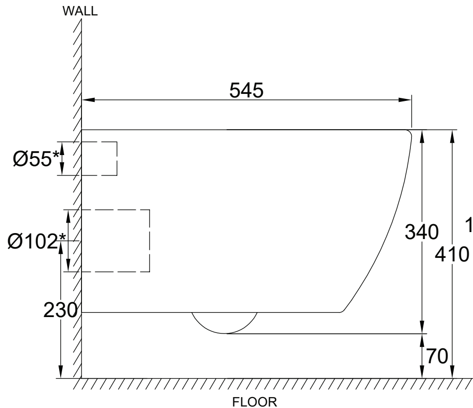
SIDE VIEW
